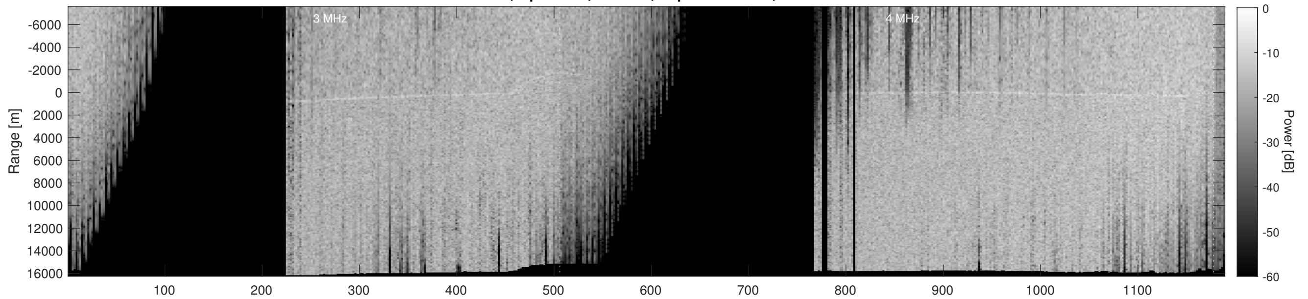
Orbit 3643, Depth-Corrected Cluttergram
