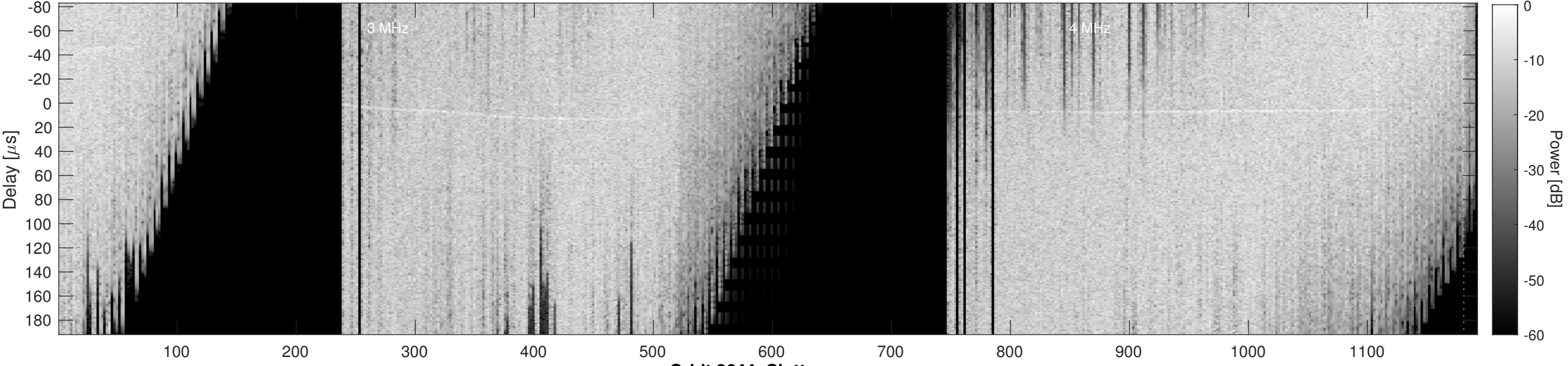
Orbit 3644, Cluttergram
