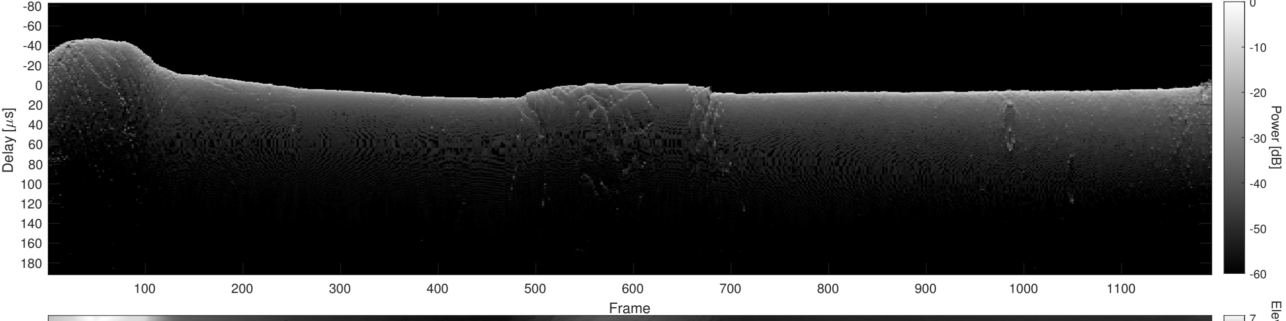
Orbit 3644, Cluttergram
