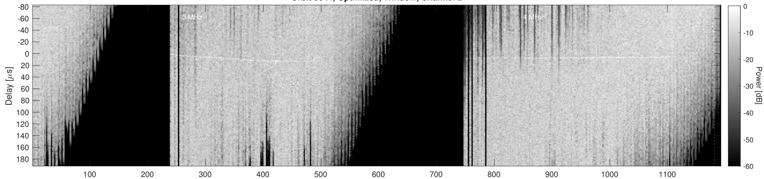
Orbit 3644, Cluttergram
