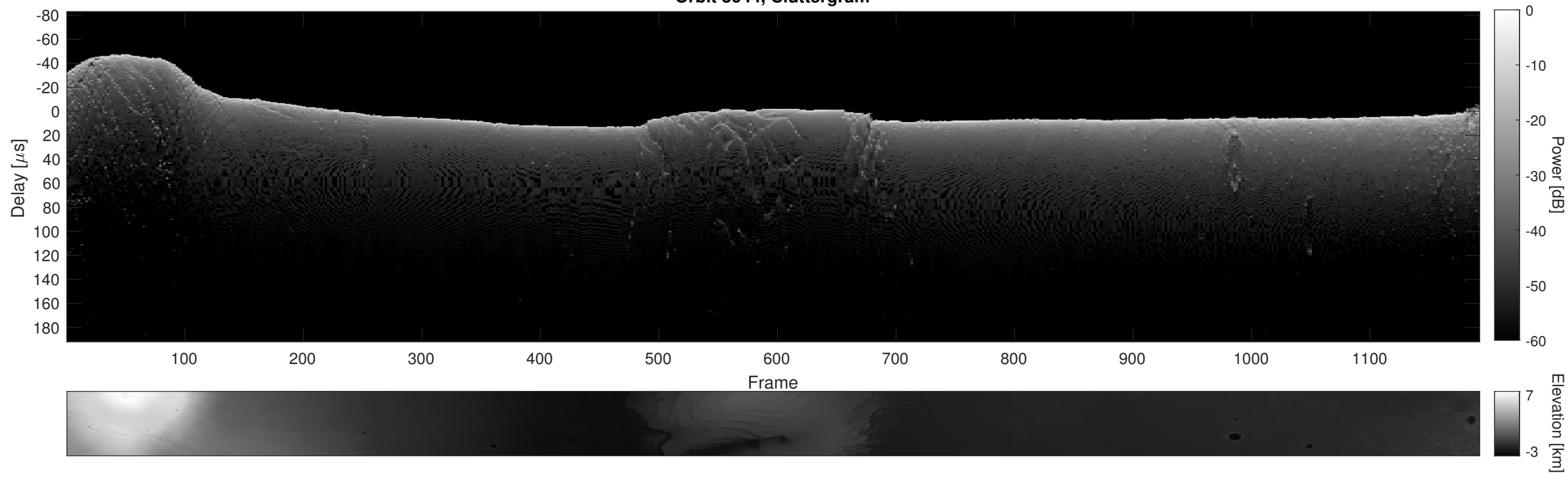
Orbit 3644, Cluttergram
