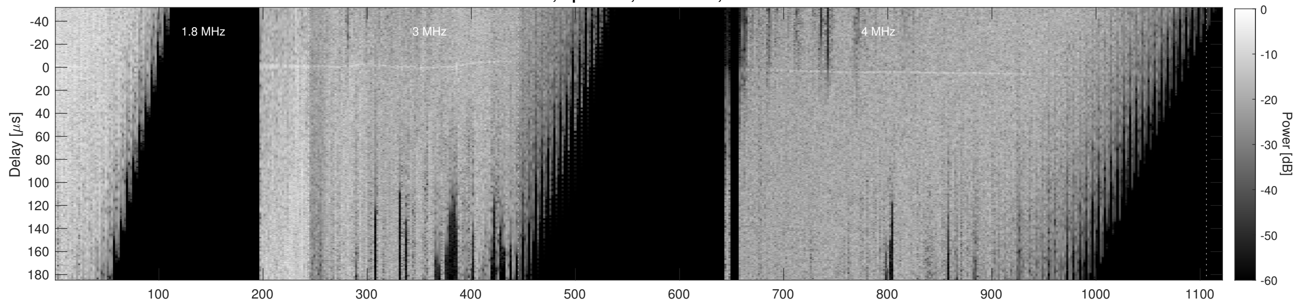
Orbit 3645, Cluttergram
