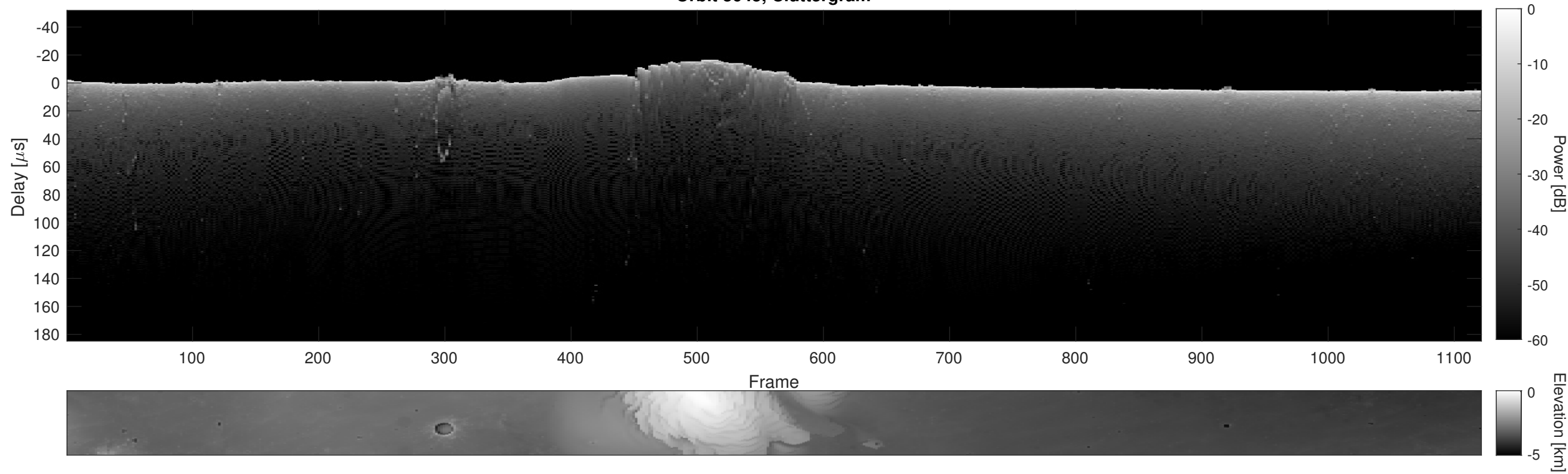
Orbit 3645, Cluttergram
