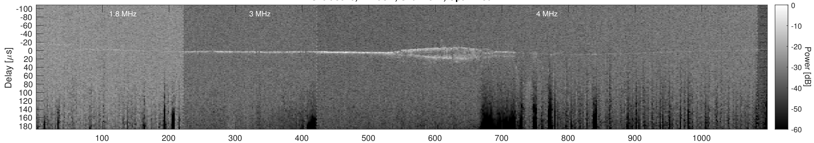
Orbit 3646, Cluttergram
