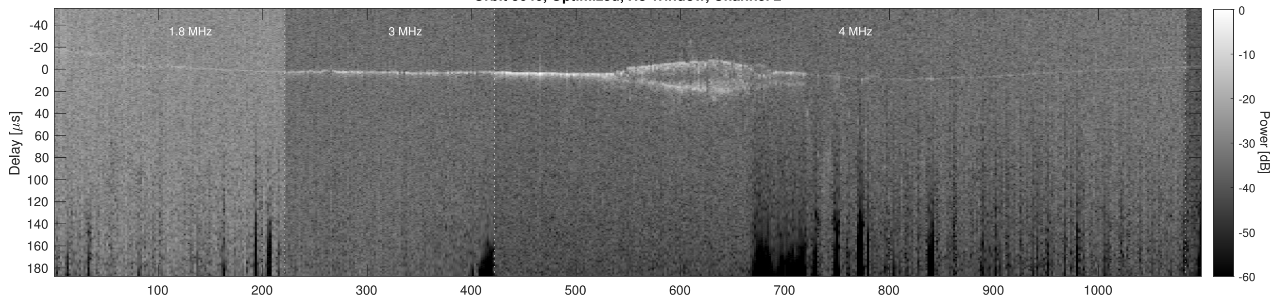
Orbit 3646, Cluttergram
