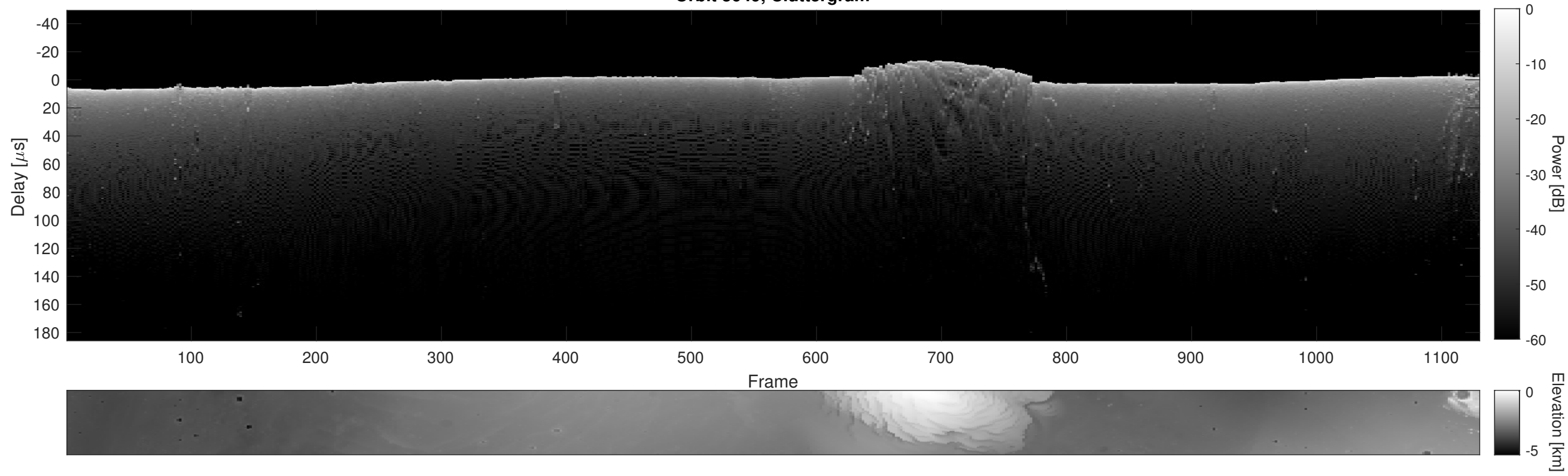
Orbit 3649, Cluttergram
