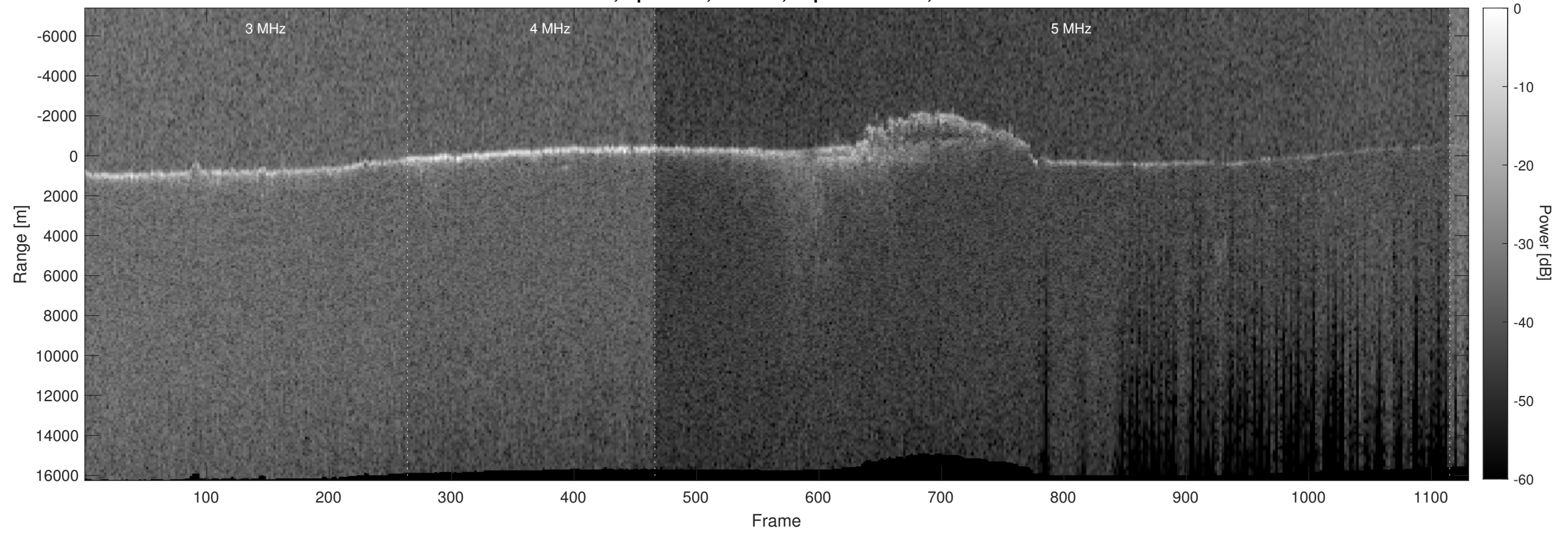
Orbit 3649, Optimized, Window, Depth-Corrected, Channel 2
