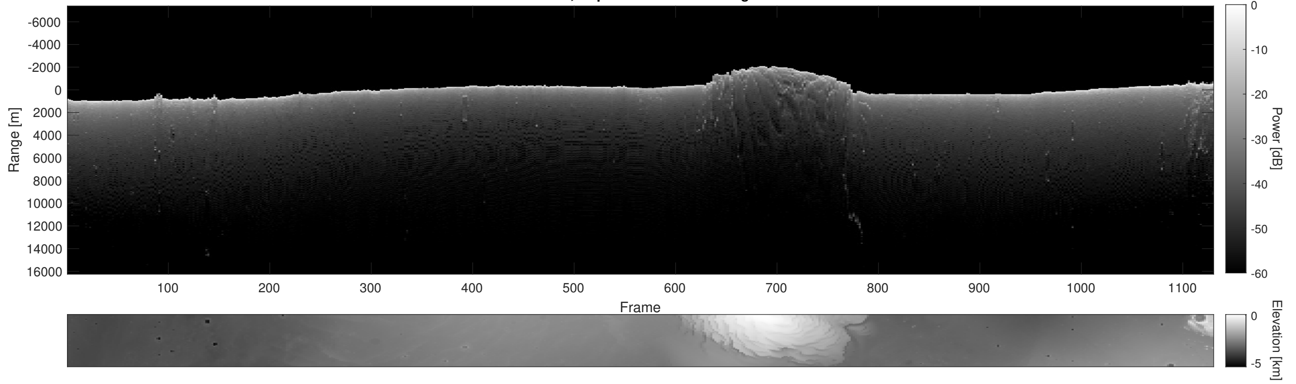
Orbit 3649, Depth-Corrected Cluttergram
