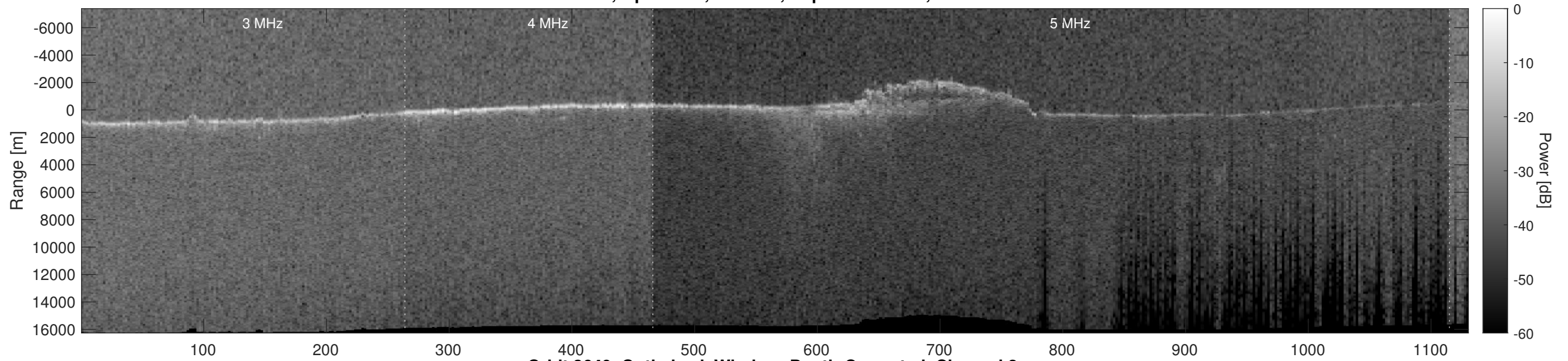
Orbit 3649, Optimized, Window, Depth-Corrected, Channel 2
