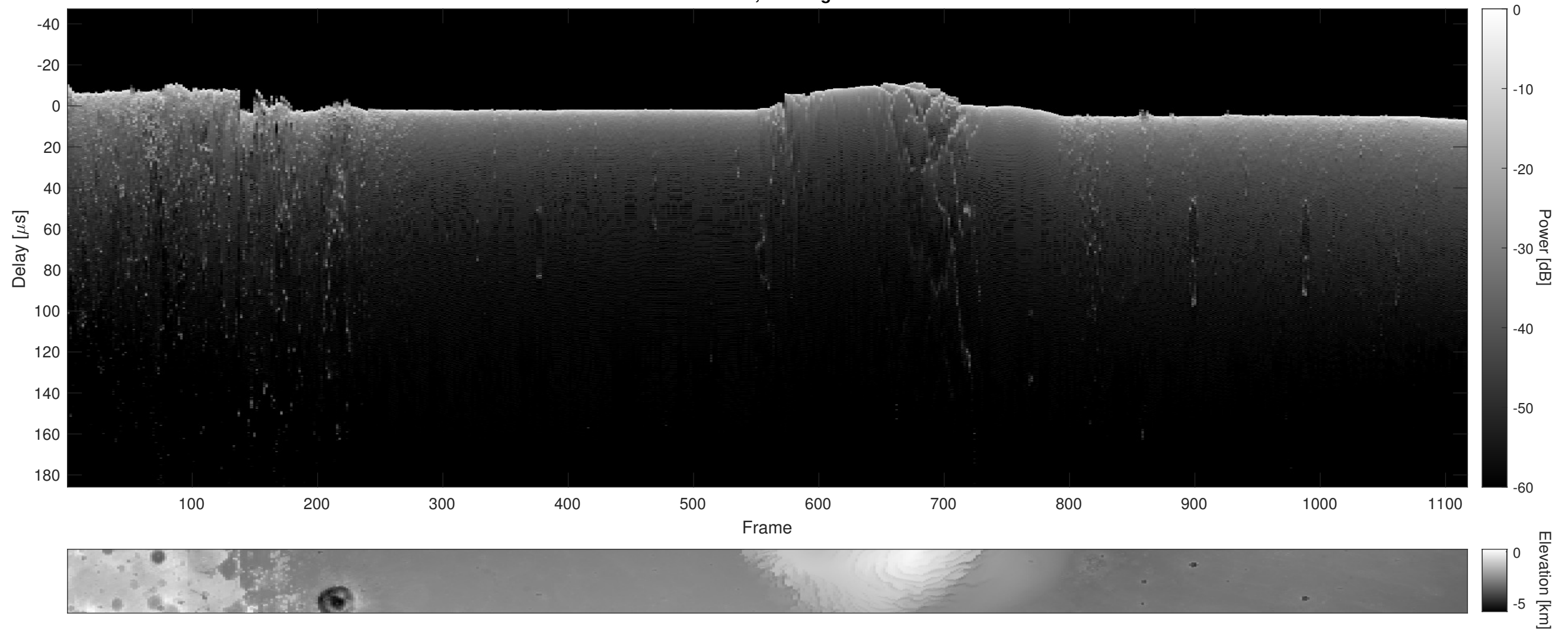
Orbit 3650, Cluttergram
