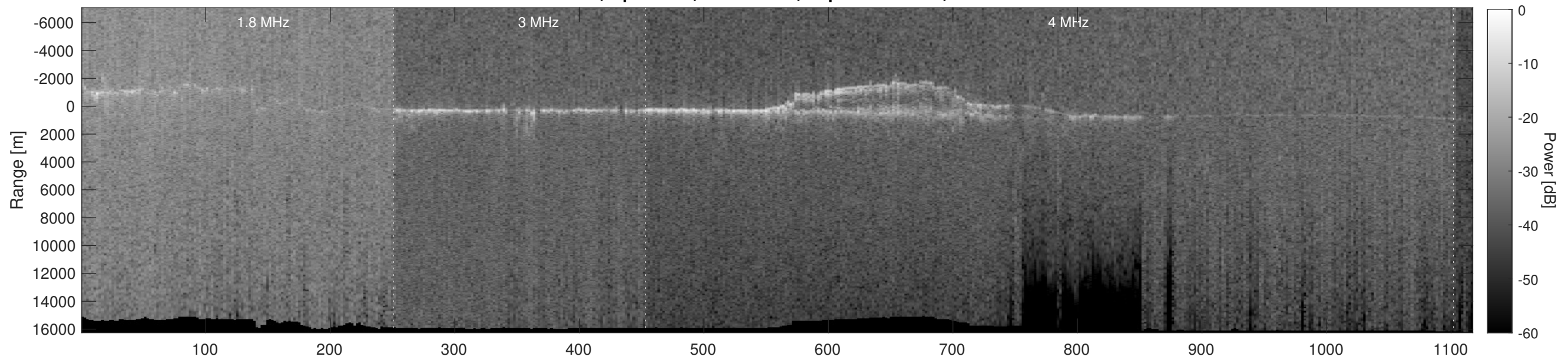
Orbit 3650, Depth-Corrected Cluttergram
