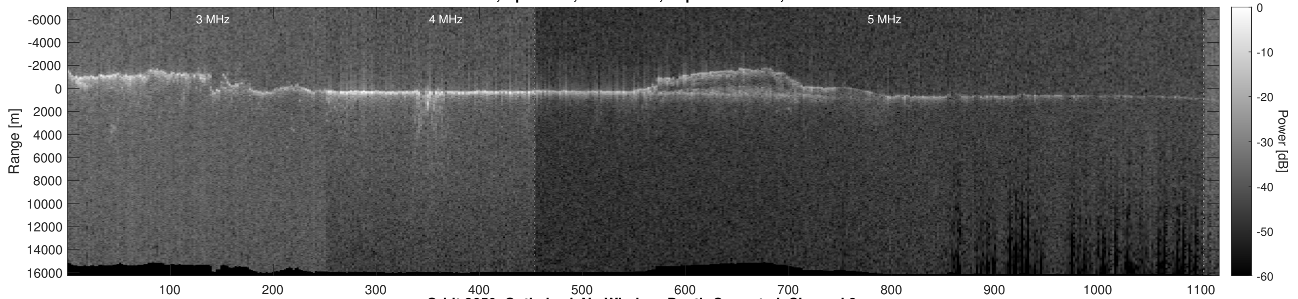
Orbit 3650, Optimized, No Window, Depth-Corrected, Channel 2
