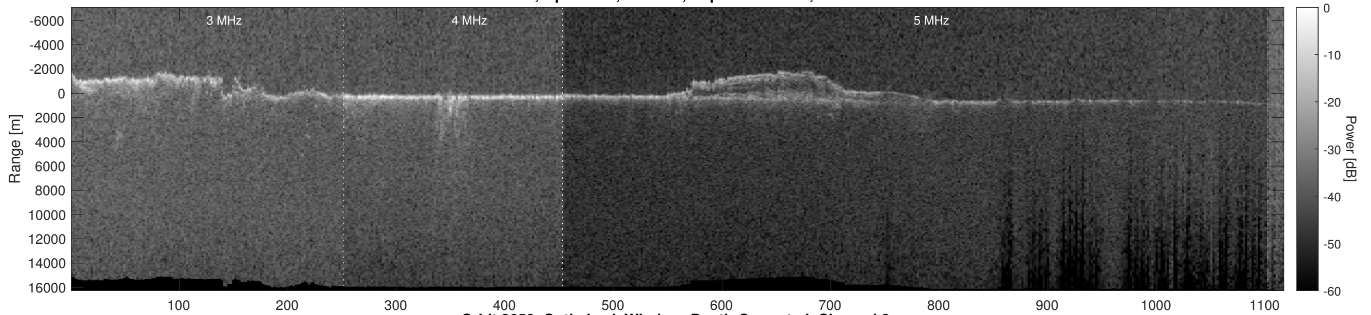
Orbit 3650, Optimized, Window, Depth-Corrected, Channel 2
