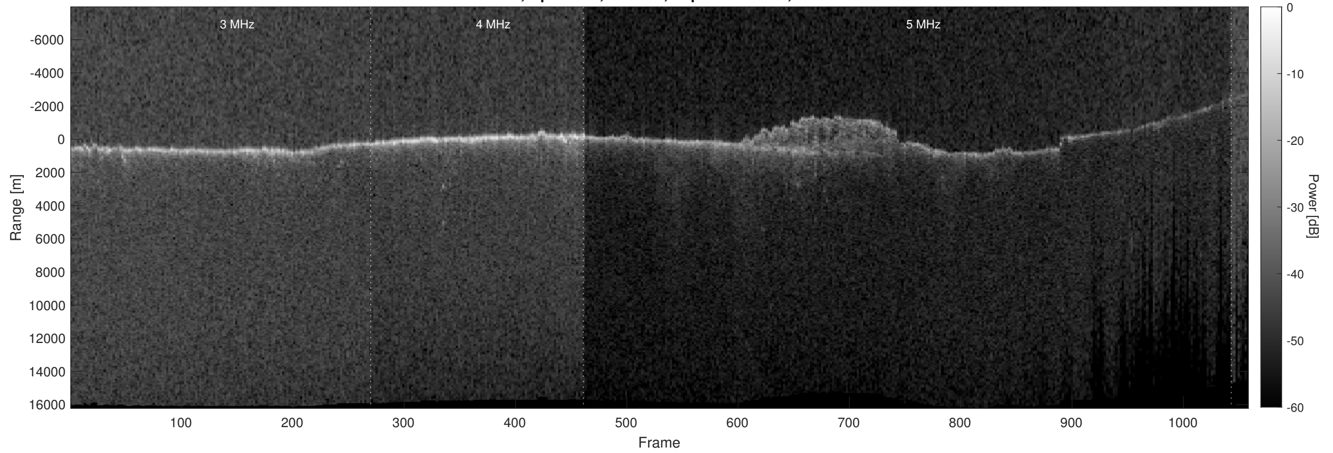
Orbit 3653, Optimized, Window, Depth-Corrected, Channel 2
