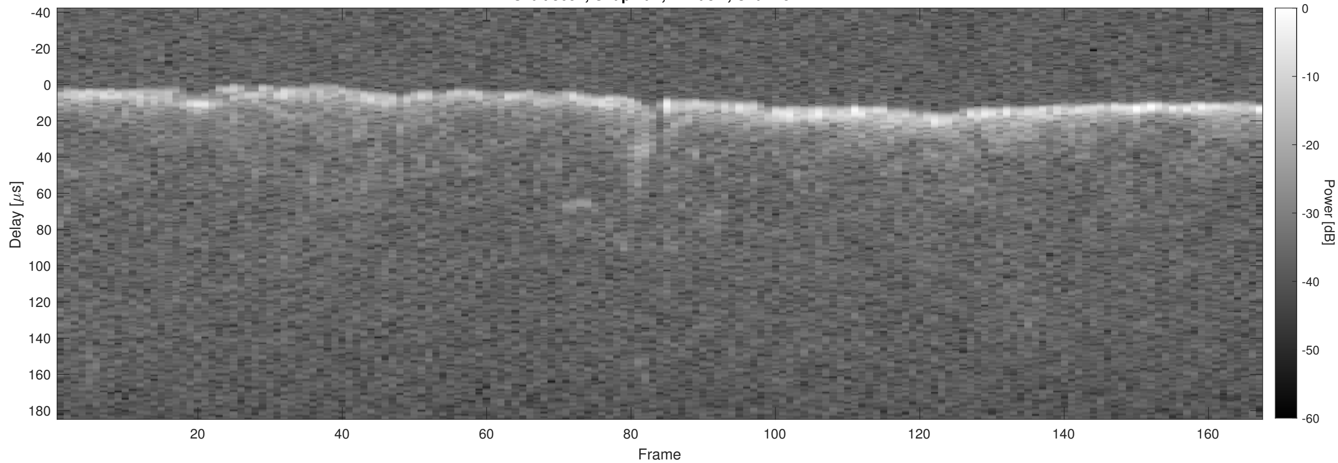
Orbit 3654, Chapman, Window, Channel 2
