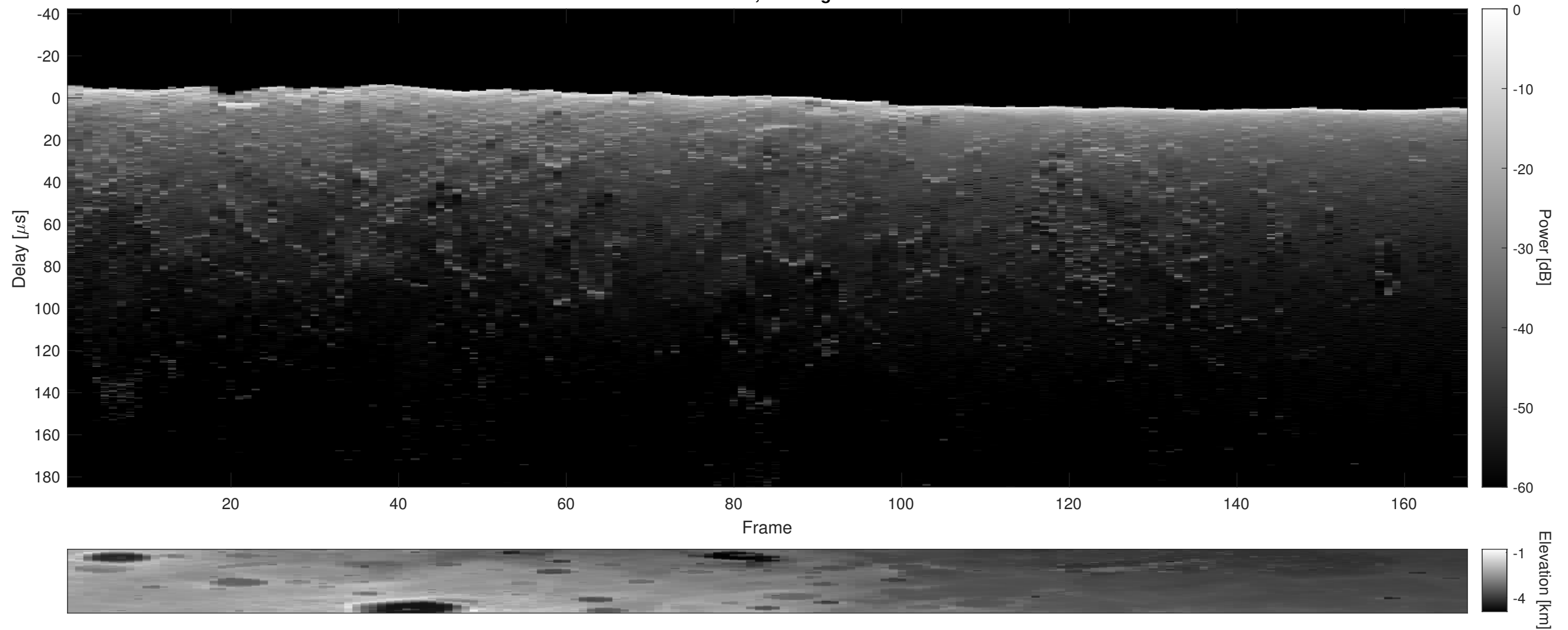
Orbit 3654, Cluttergram
