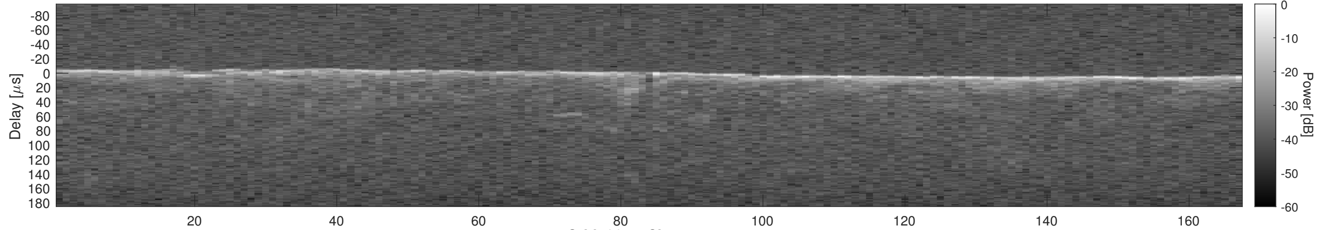
Orbit 3654, Cluttergram
