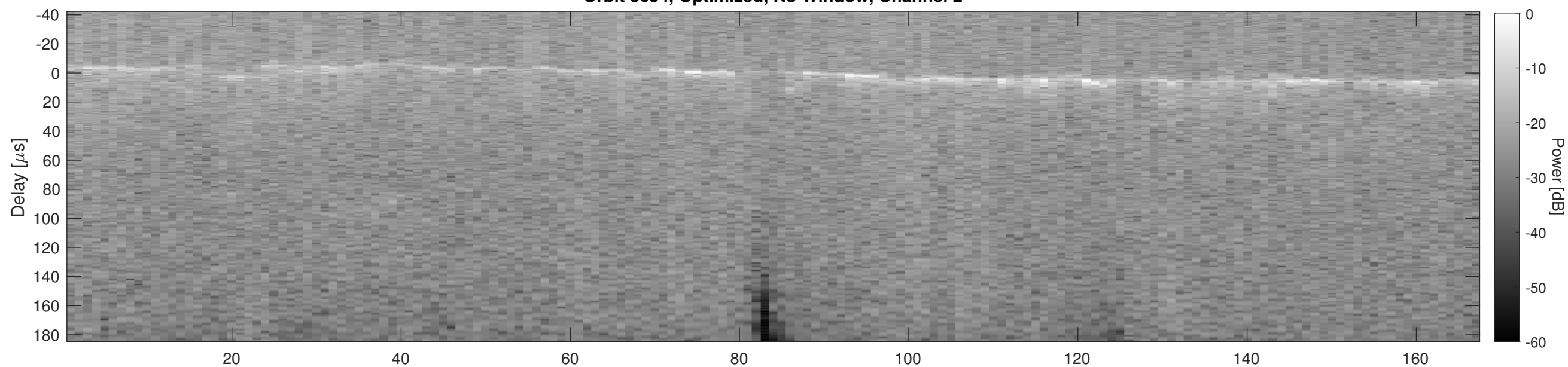
Orbit 3654, Cluttergram
