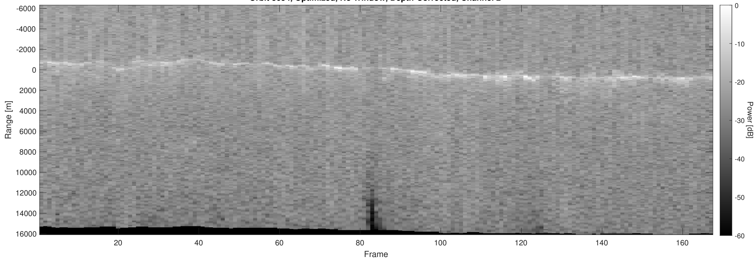
Orbit 3654, Optimized, No Window, Depth-Corrected, Channel 2
