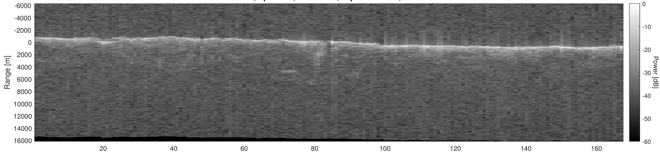
Orbit 3654, Optimized, No Window, Depth-Corrected, Channel 2
