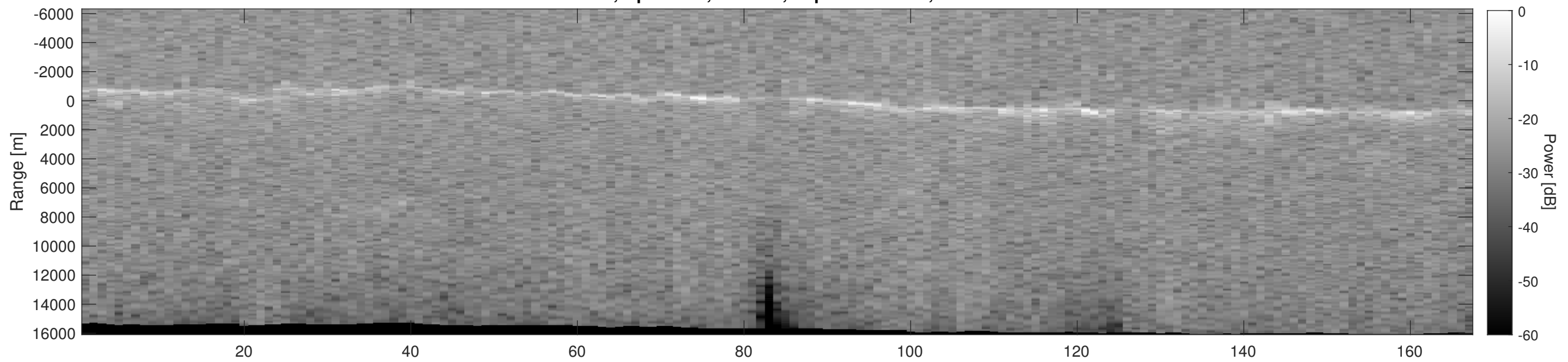
Orbit 3654, Depth-Corrected Cluttergram
