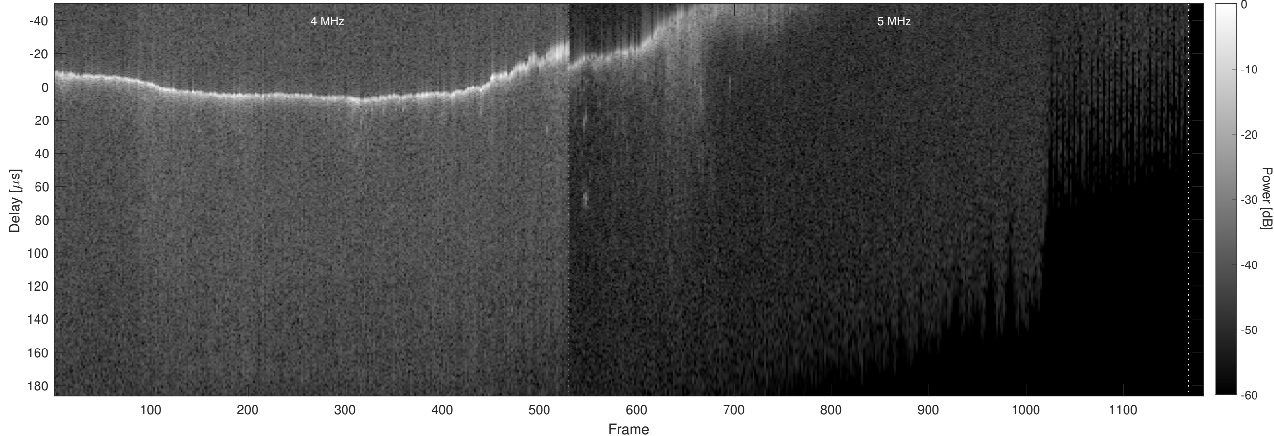
Orbit 3656, Chapman, No Window, Channel 2
