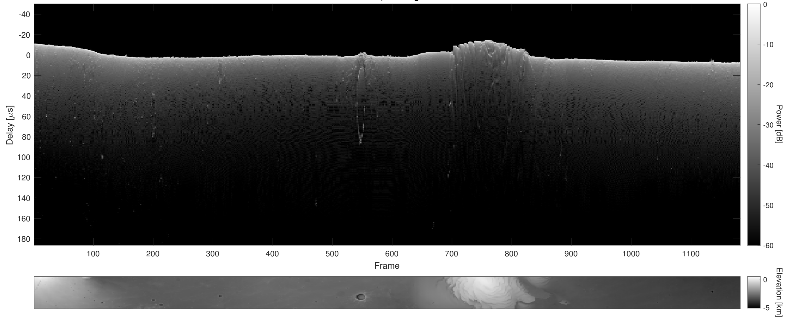
Orbit 3656, Cluttergram
