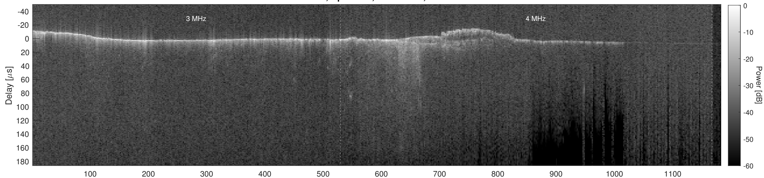
Orbit 3656, Cluttergram
