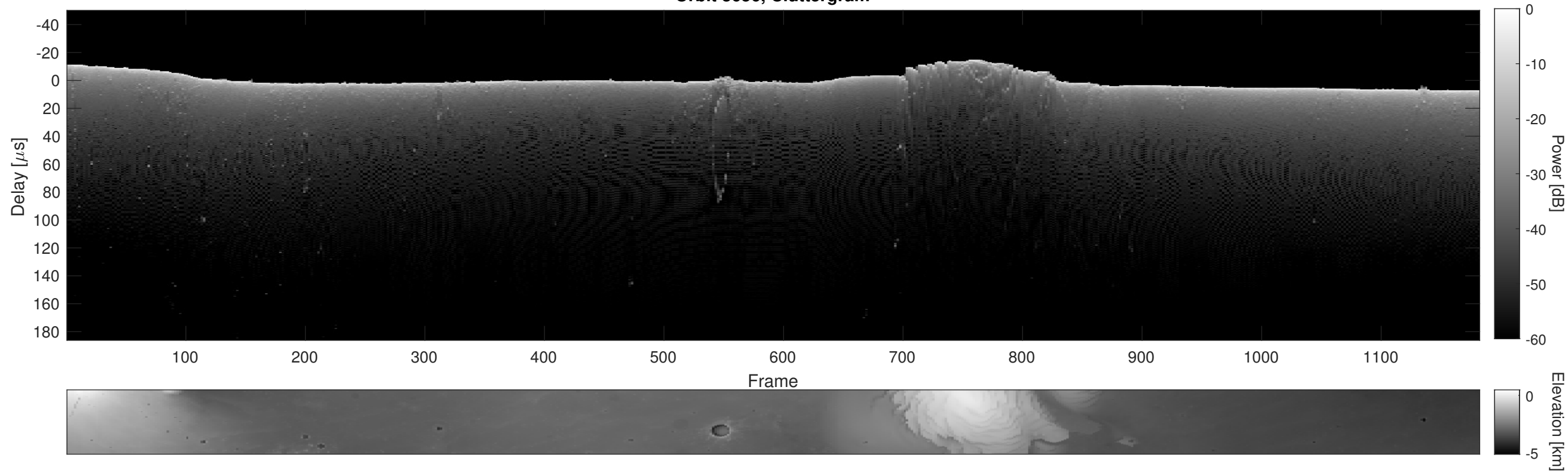
Orbit 3656, Cluttergram
