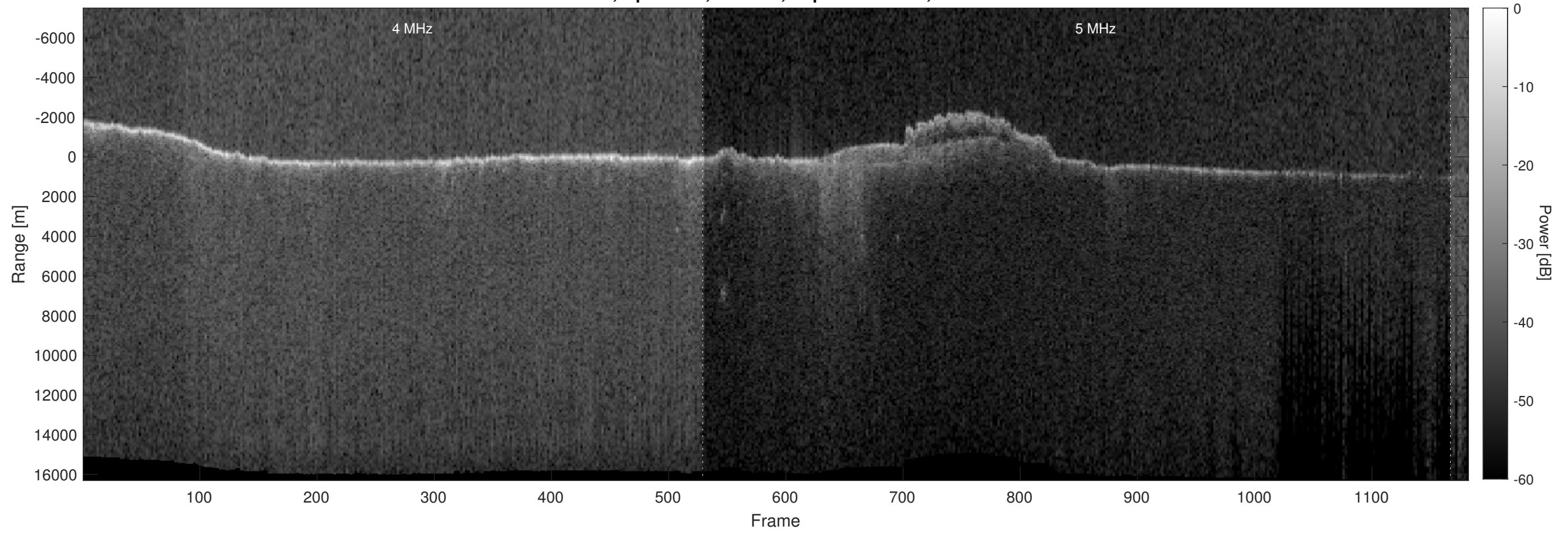
Orbit 3656, Optimized, Window, Depth-Corrected, Channel 2
