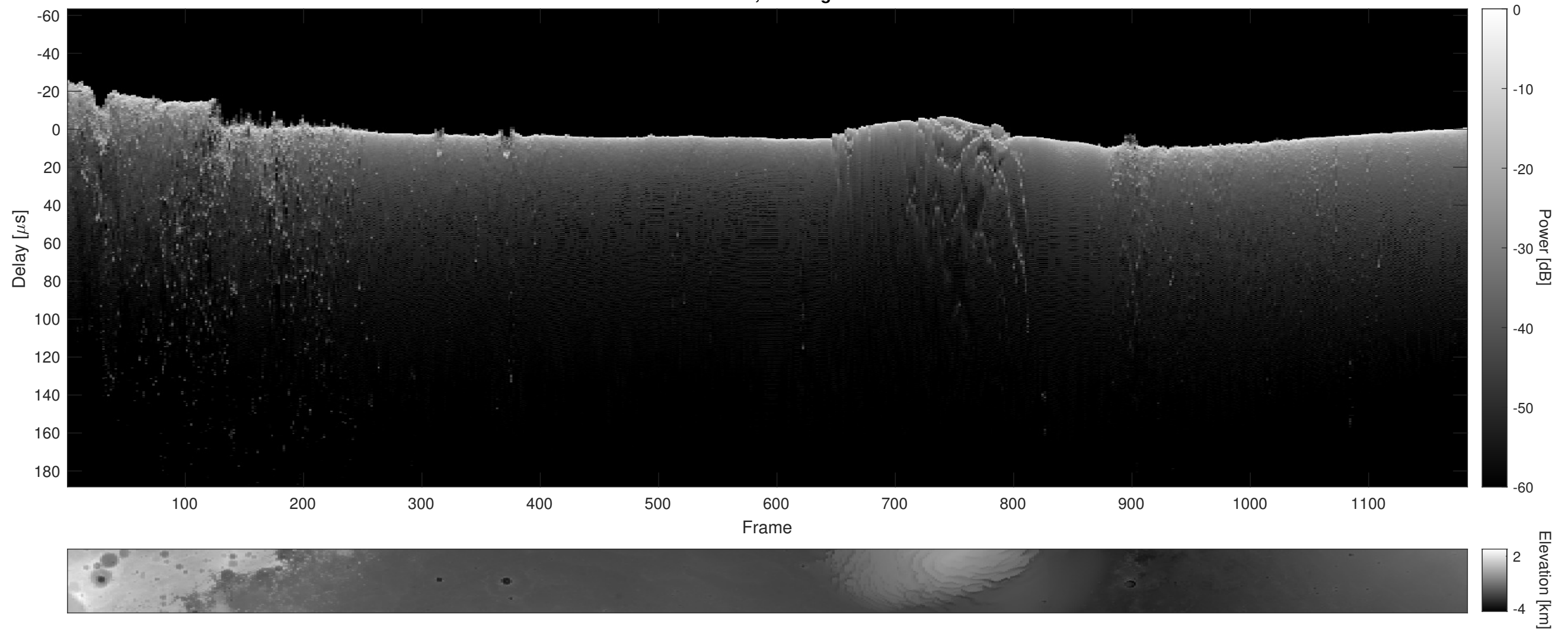
Orbit 3657, Cluttergram
