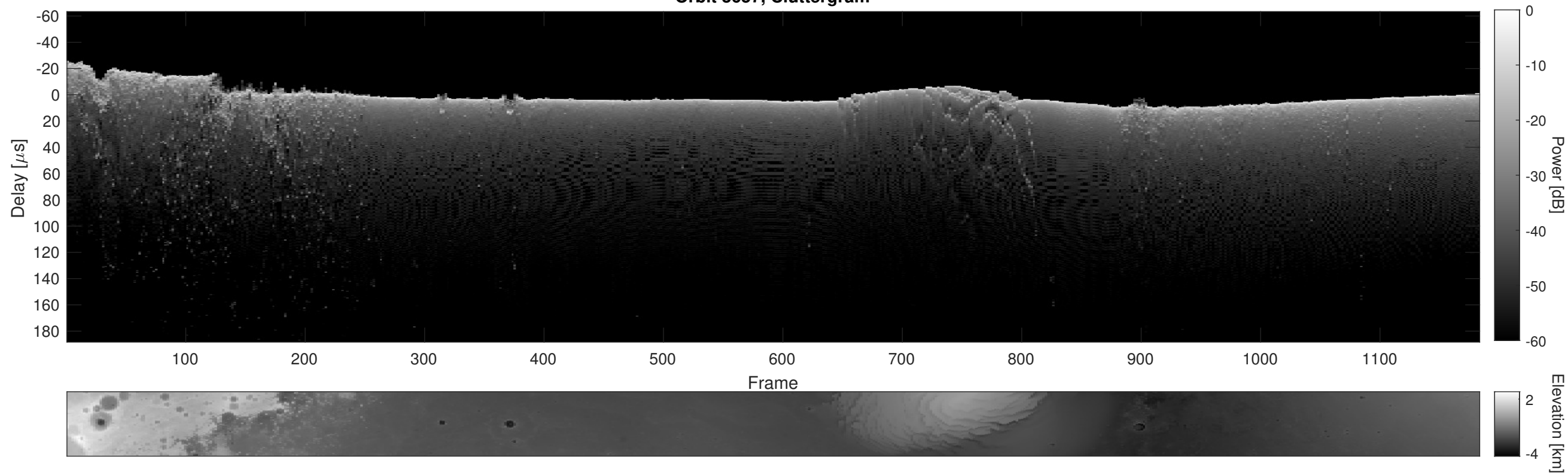
Orbit 3657, Cluttergram
