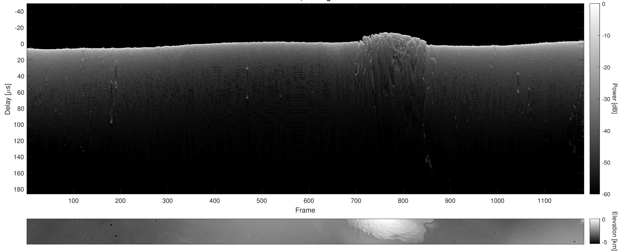
Orbit 3660, Cluttergram
