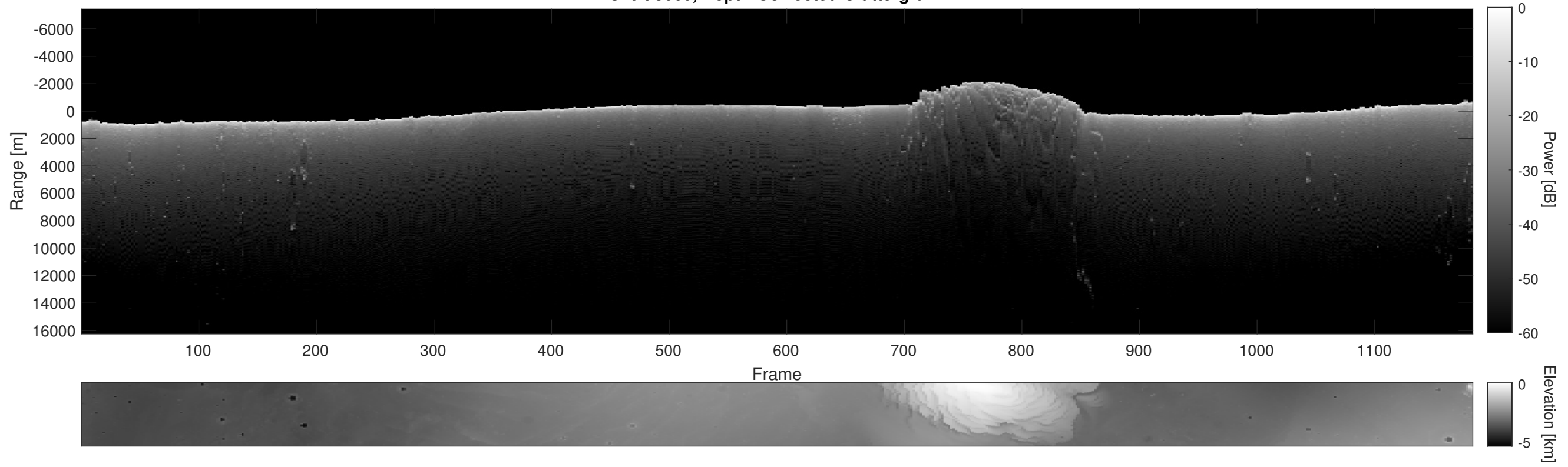
Orbit 3660, Depth-Corrected Cluttergram
