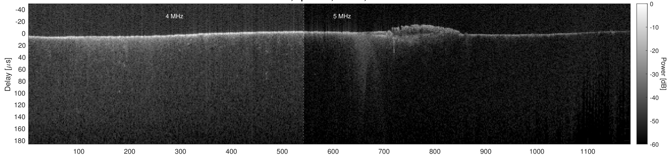
Orbit 3660, Optimized, Window, Channel 2
