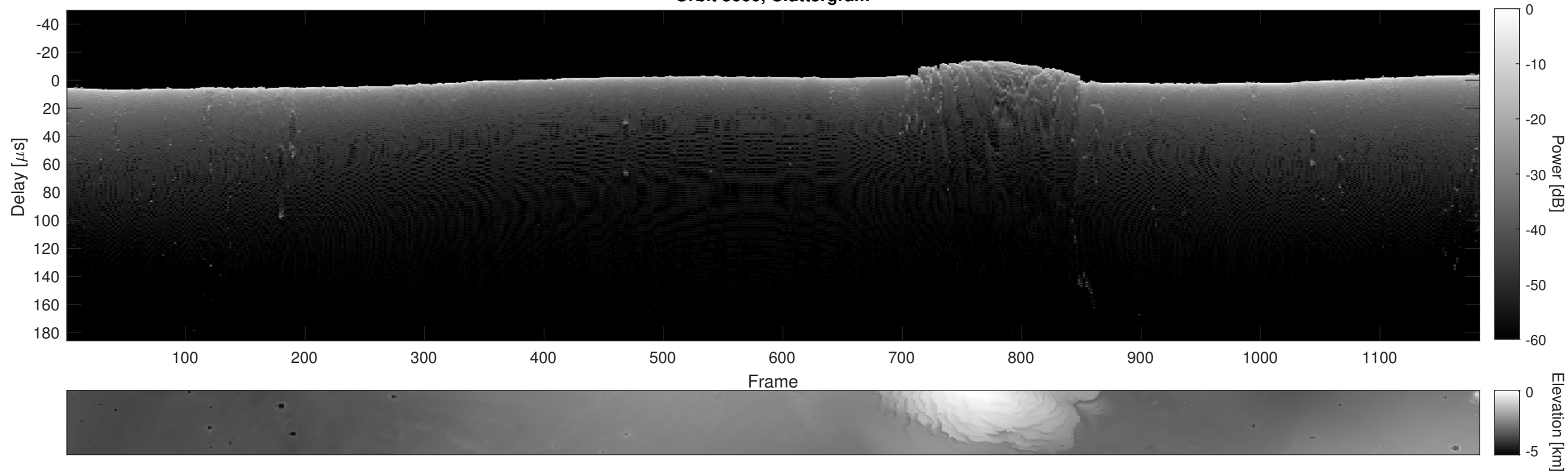
Orbit 3660, Cluttergram
