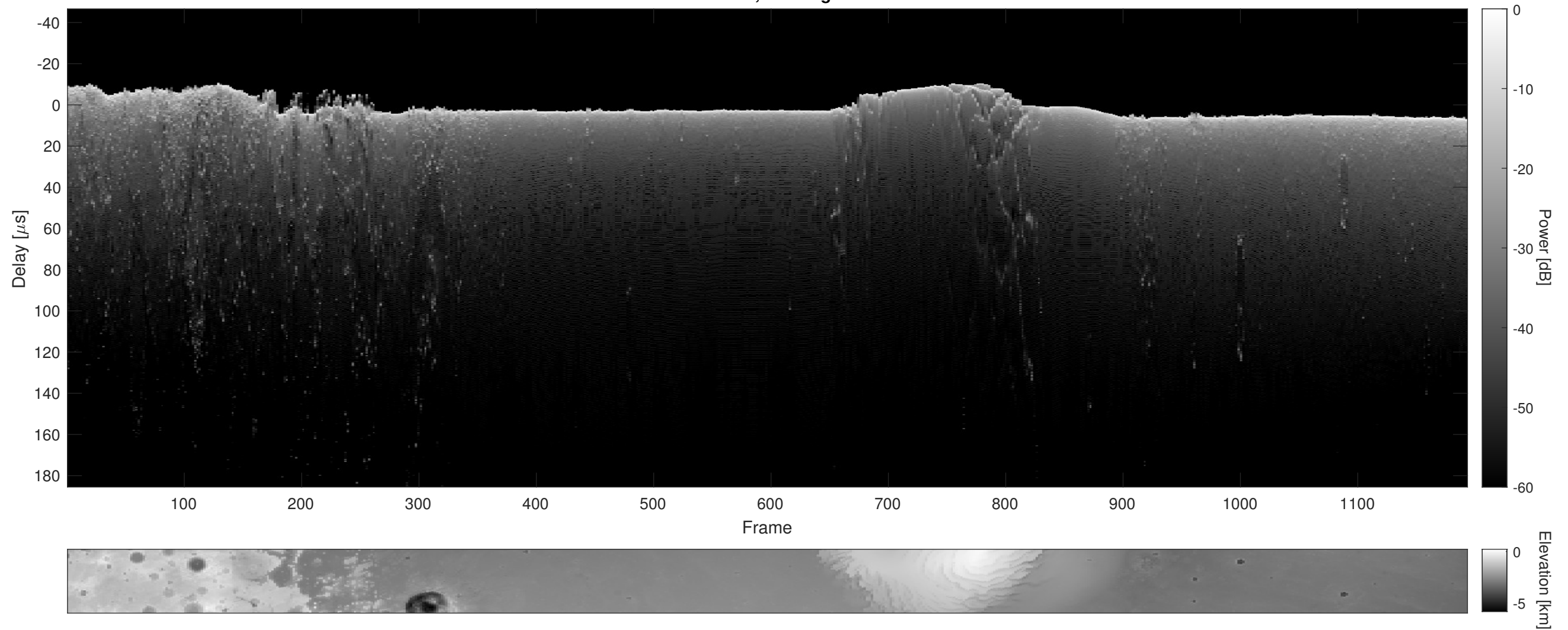
Orbit 3661, Cluttergram
