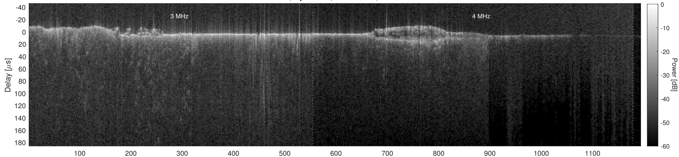
Orbit 3661, Cluttergram
