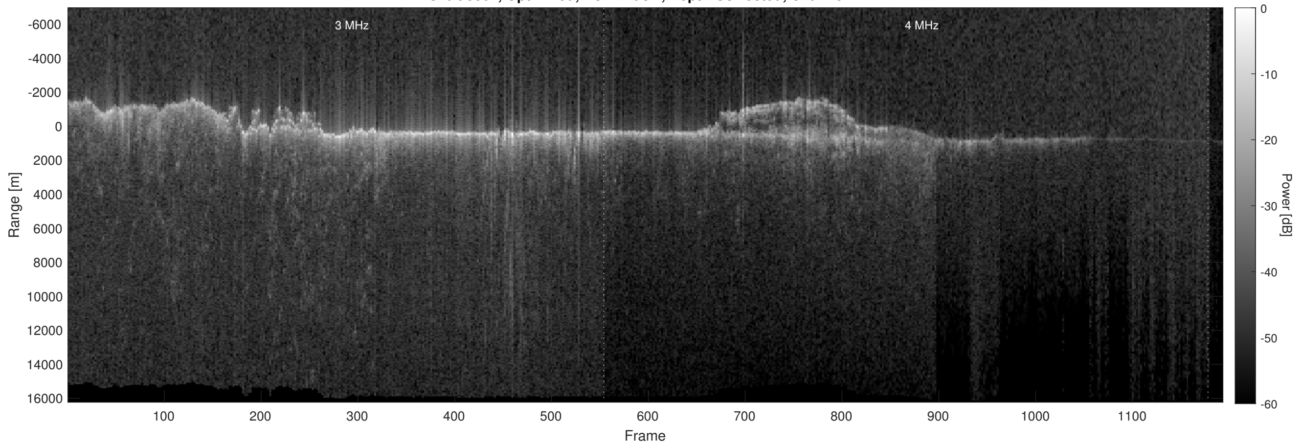
Orbit 3661, Optimized, No Window, Depth-Corrected, Channel 2
