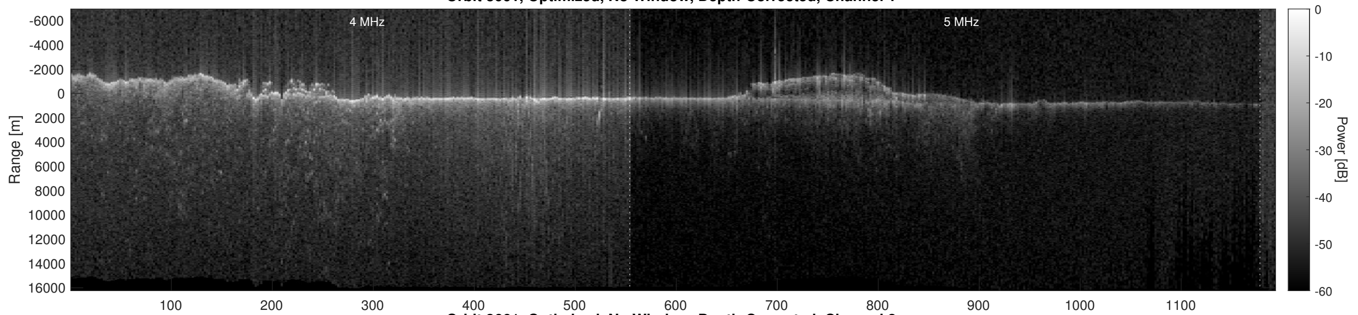
Orbit 3661, Optimized, No Window, Depth-Corrected, Channel 2
