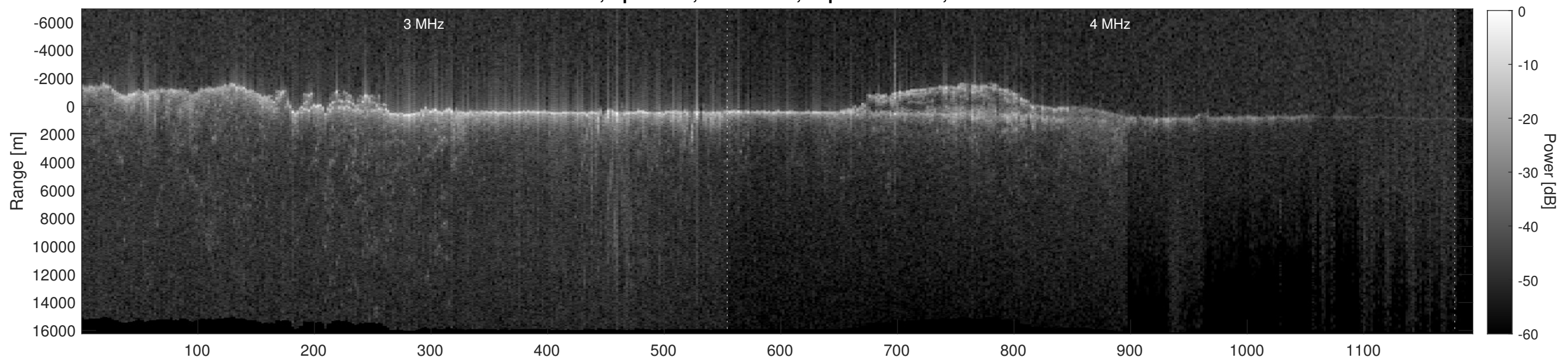
Orbit 3661, Depth-Corrected Cluttergram
