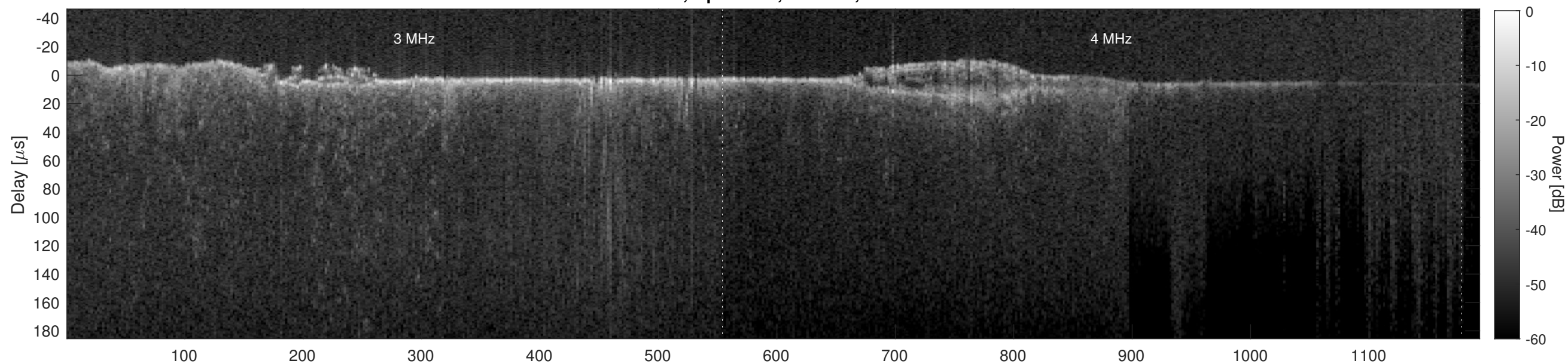
Orbit 3661, Cluttergram
