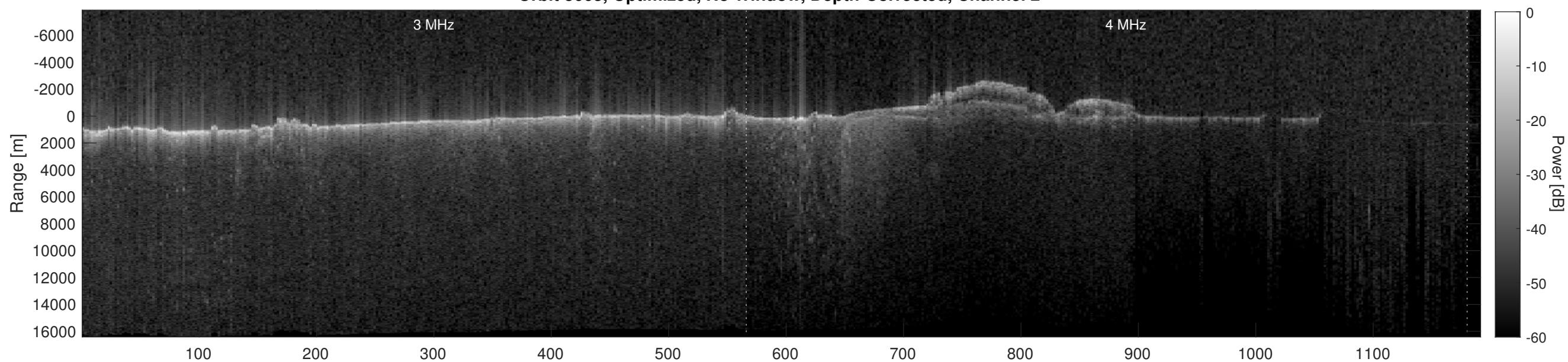
Orbit 3663, Depth-Corrected Cluttergram
