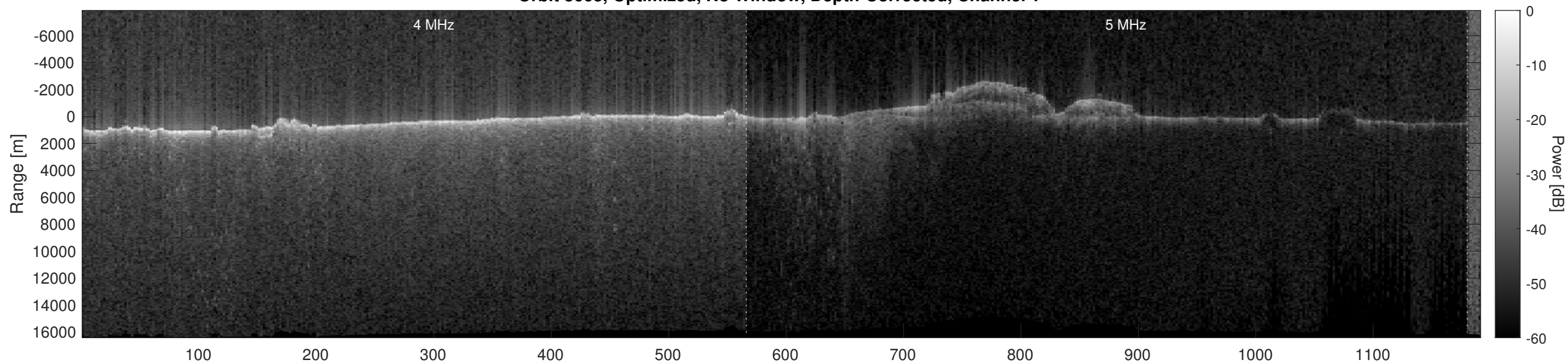
Orbit 3663, Optimized, No Window, Depth-Corrected, Channel 2
