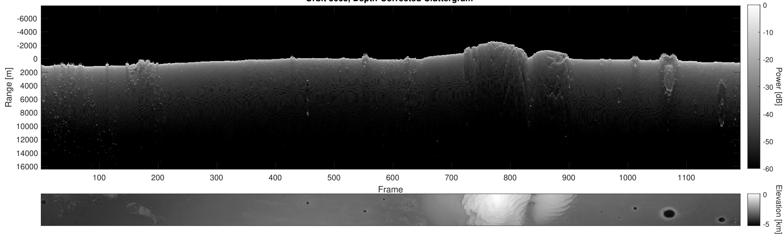
Orbit 3663, Depth-Corrected Cluttergram
