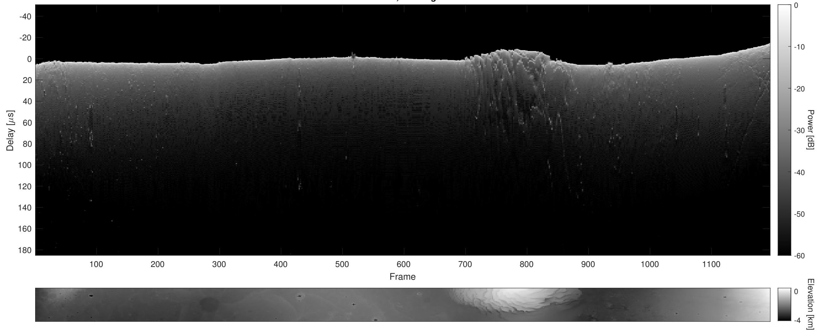
Orbit 3664, Cluttergram
