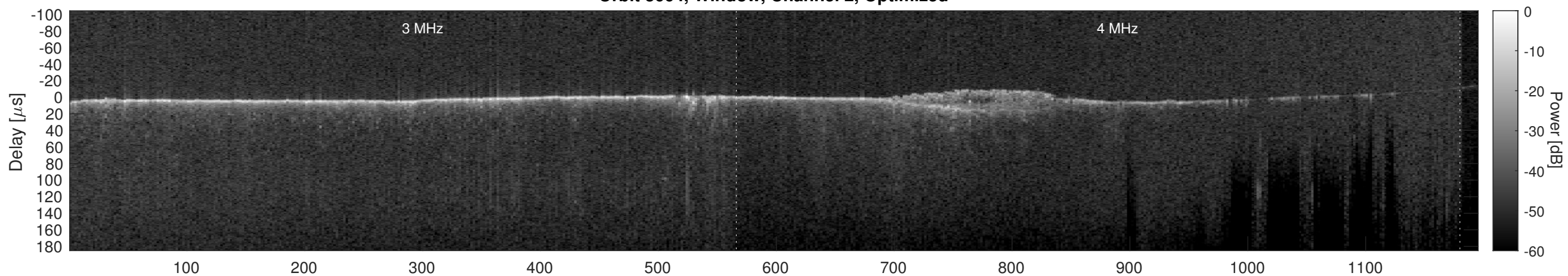
Orbit 3664, Cluttergram
