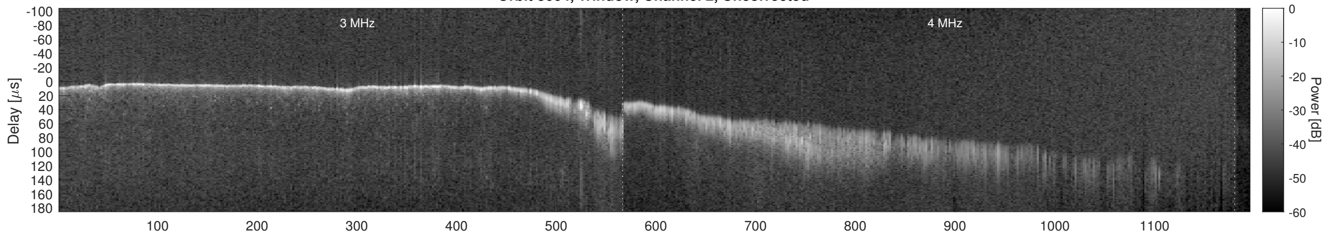
Orbit 3664, Window, Channel 2, Chapman
