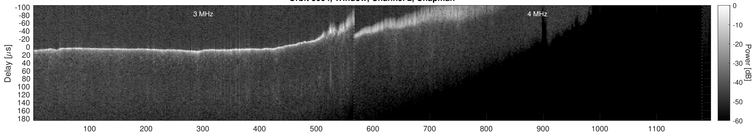
Orbit 3664, Window, Channel 2, Optimized
