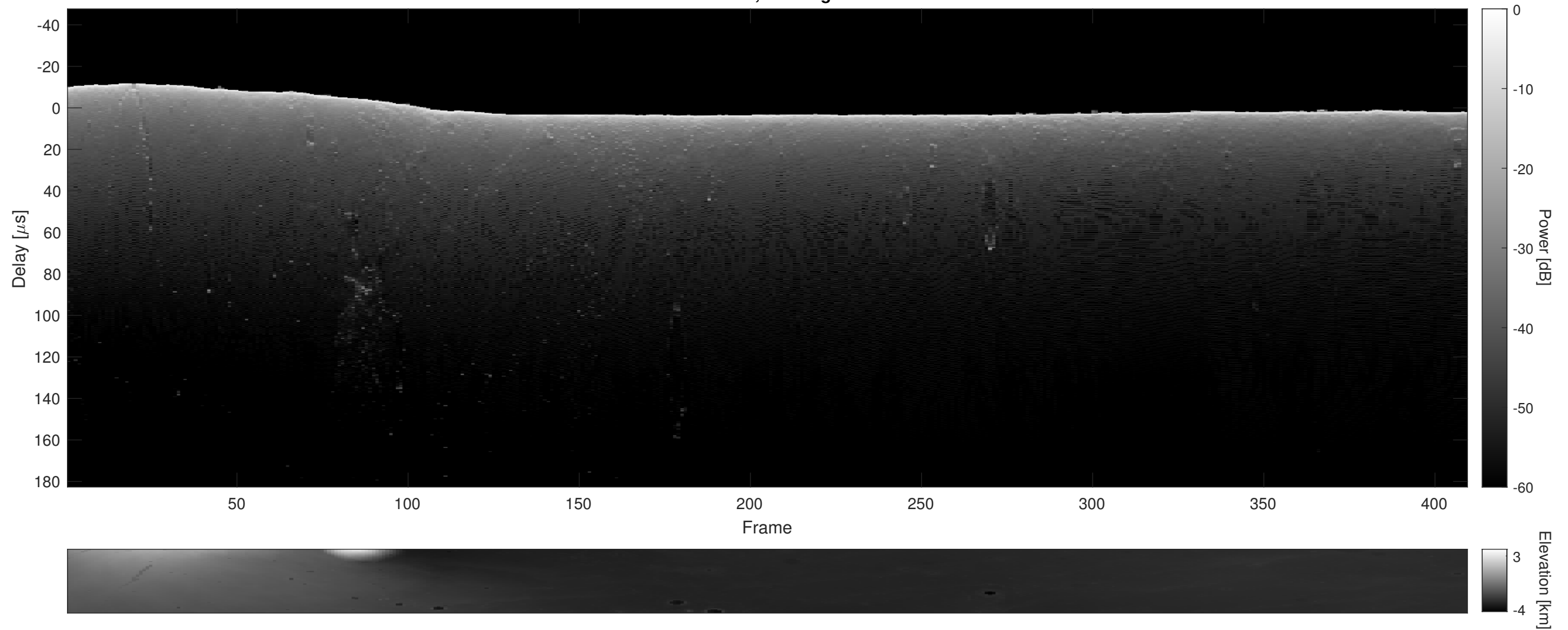
Orbit 3667, Cluttergram
