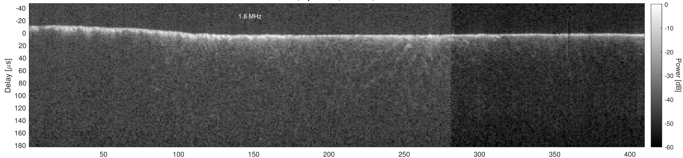
Orbit 3667, Cluttergram
