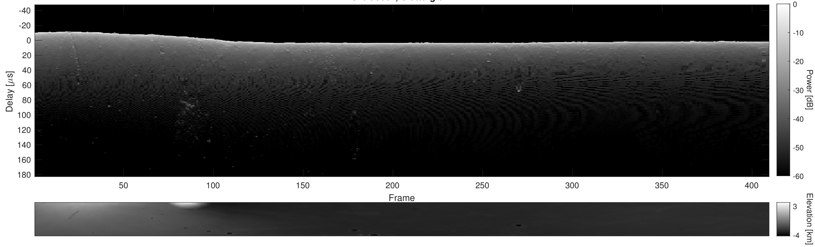
Orbit 3667, Cluttergram
