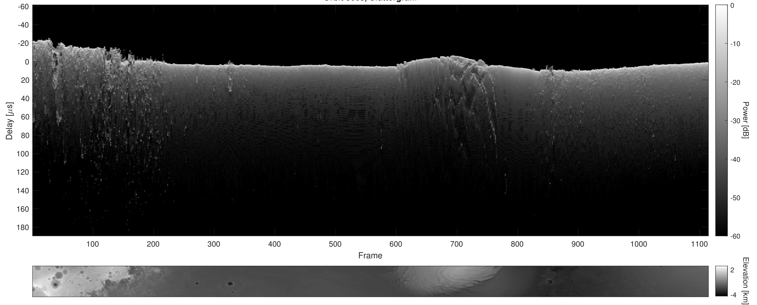
Orbit 3668, Cluttergram
