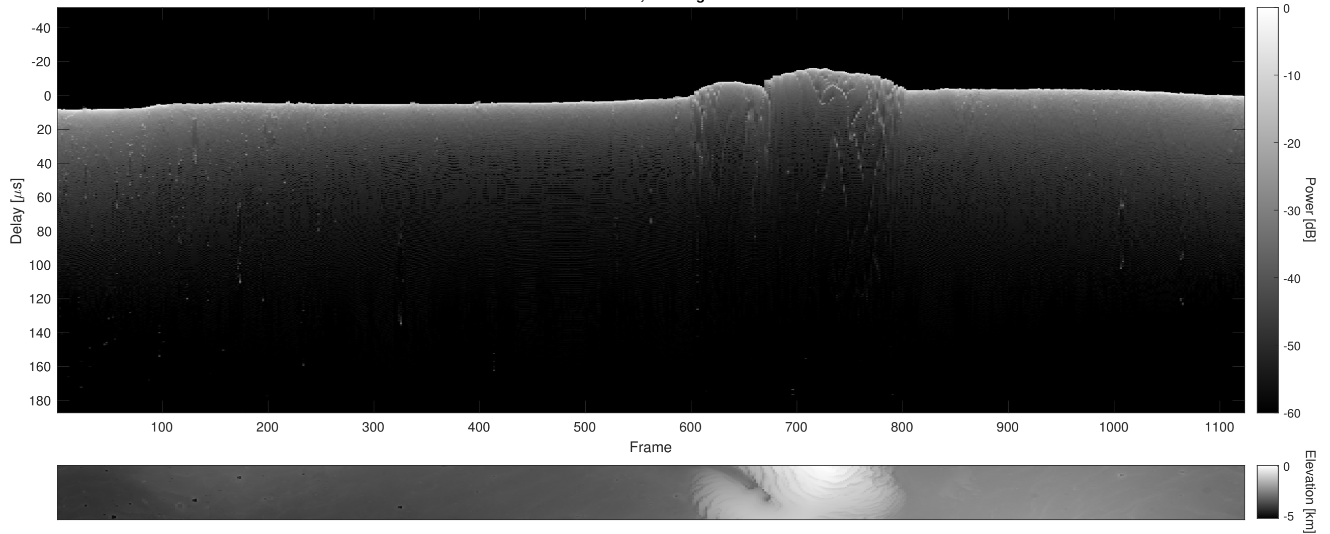
Orbit 3669, Cluttergram
