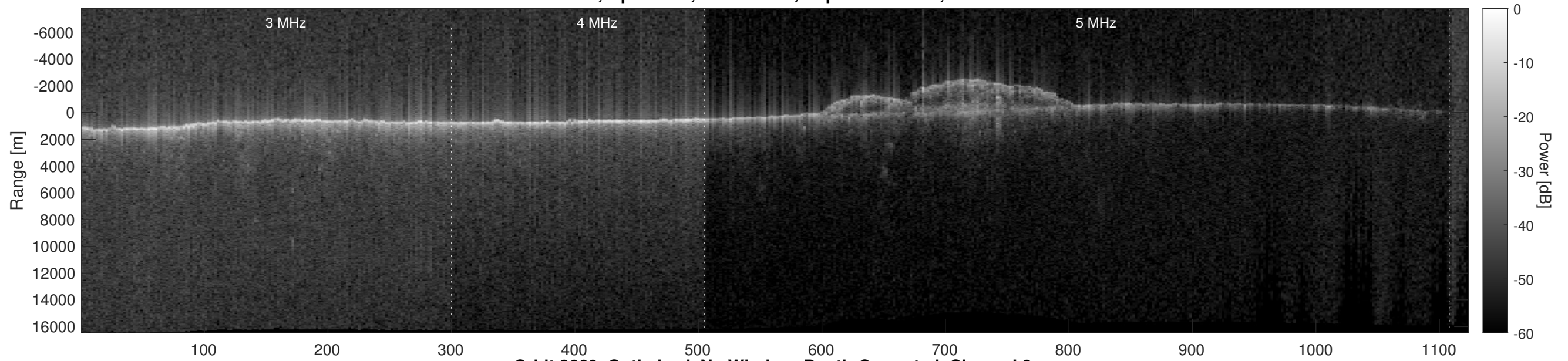
Orbit 3669, Optimized, No Window, Depth-Corrected, Channel 2
