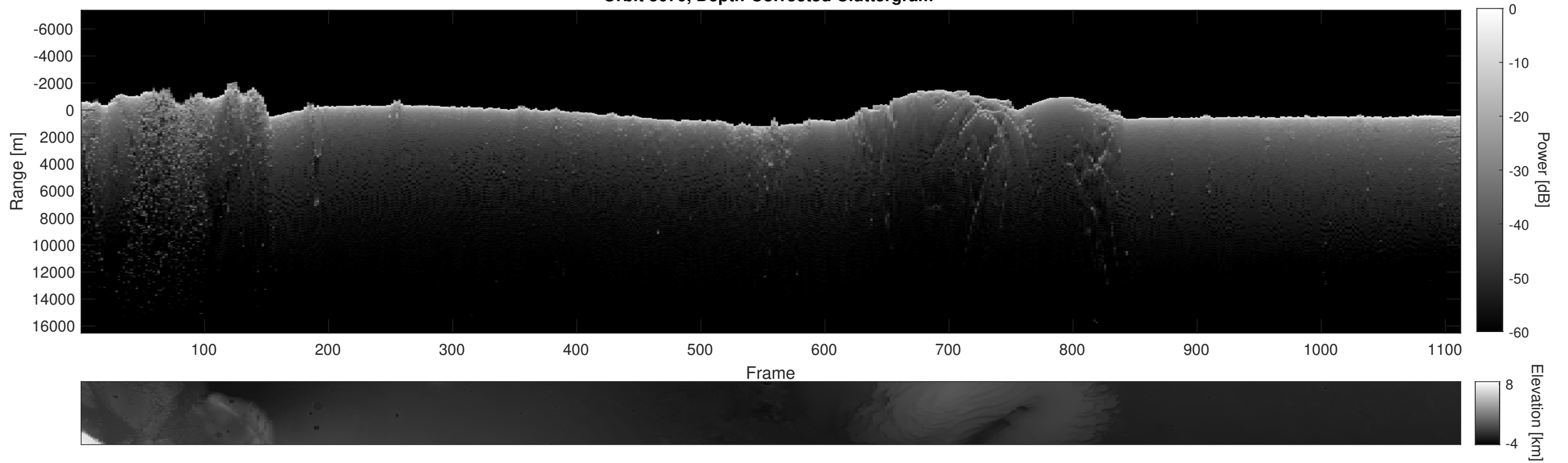
Orbit 3670, Depth-Corrected Cluttergram
