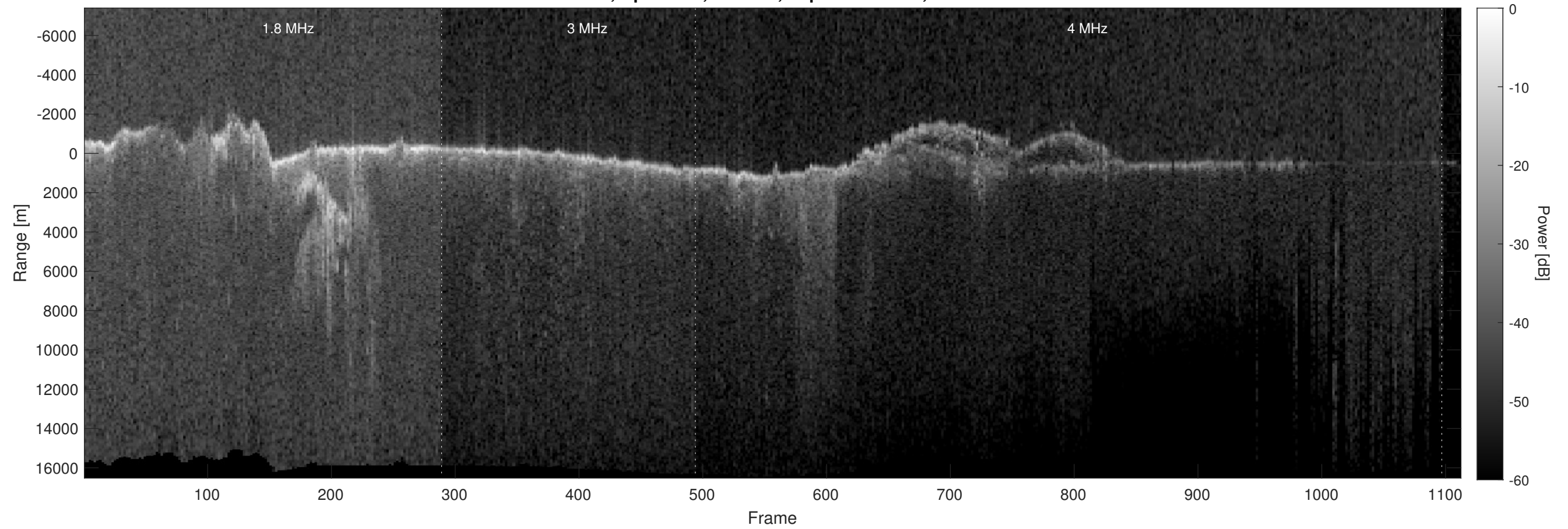
Orbit 3670, Optimized, Window, Depth-Corrected, Channel 2
