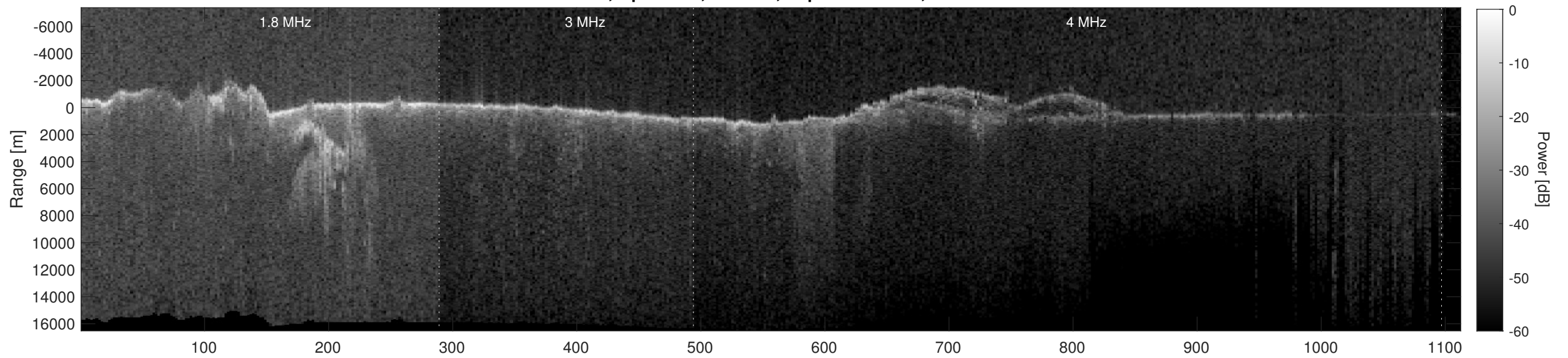
Orbit 3670, Depth-Corrected Cluttergram
