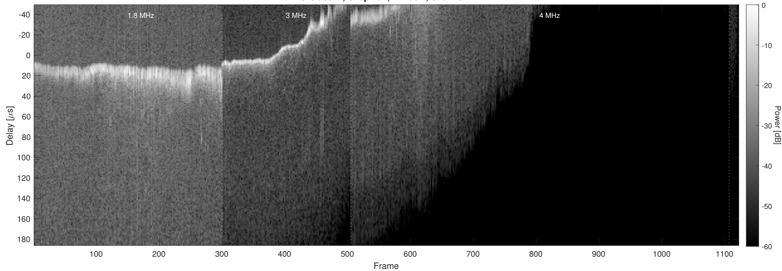
Orbit 3671, Chapman, Window, Channel 2
