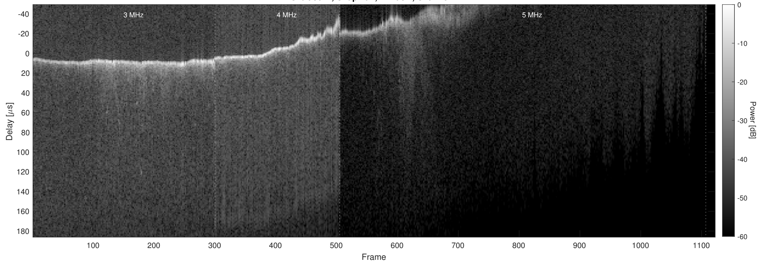
Orbit 3671, Chapman, Window, Channel 2
