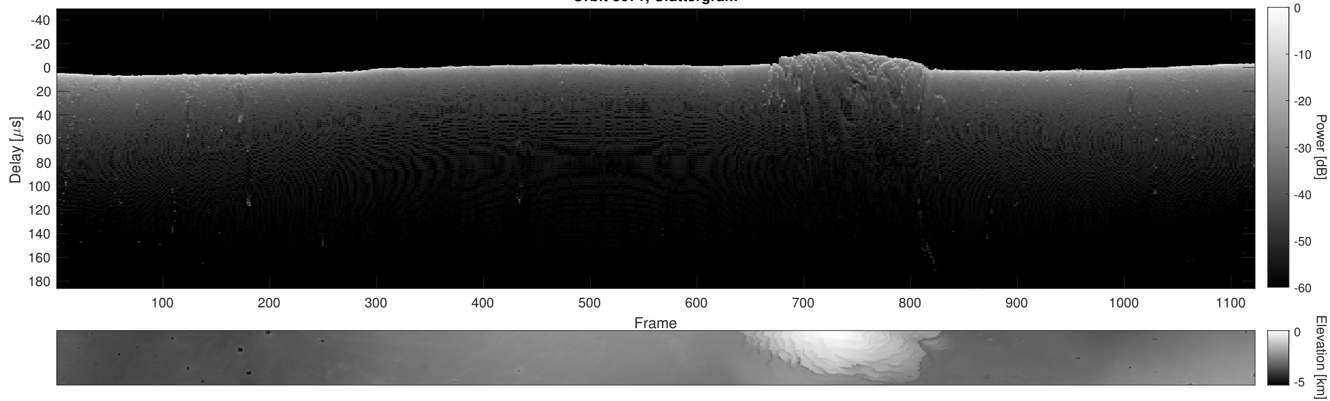
Orbit 3671, Cluttergram
