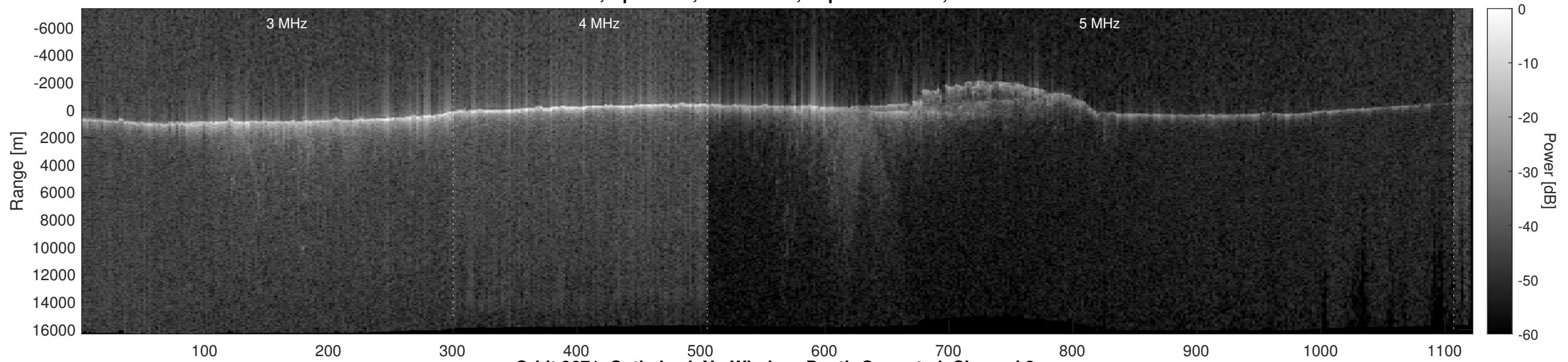
Orbit 3671, Optimized, No Window, Depth-Corrected, Channel 2
