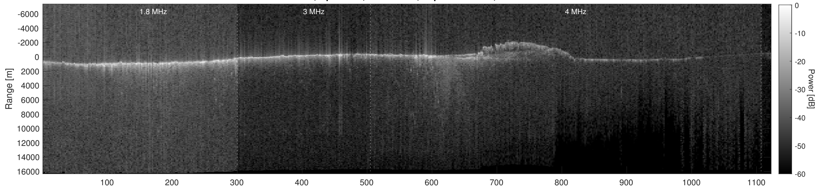
Orbit 3671, Depth-Corrected Cluttergram
