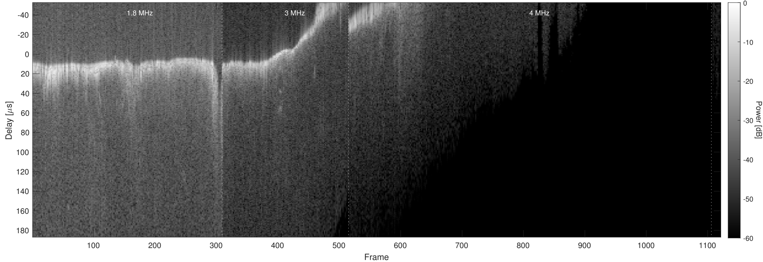
Orbit 3674, Chapman, No Window, Channel 2
